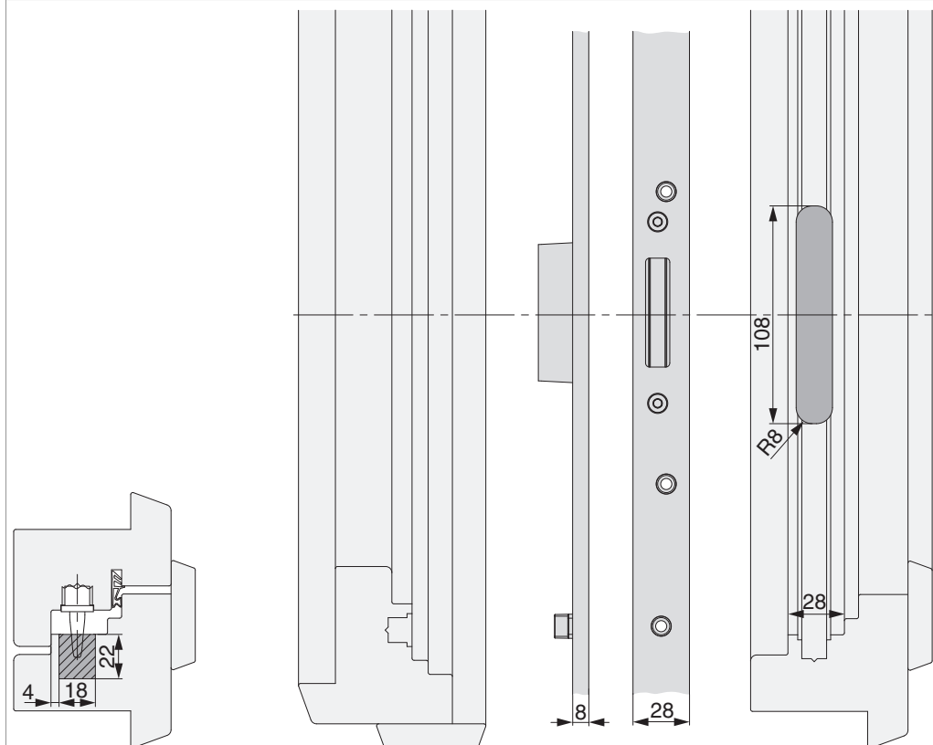
Detail A
