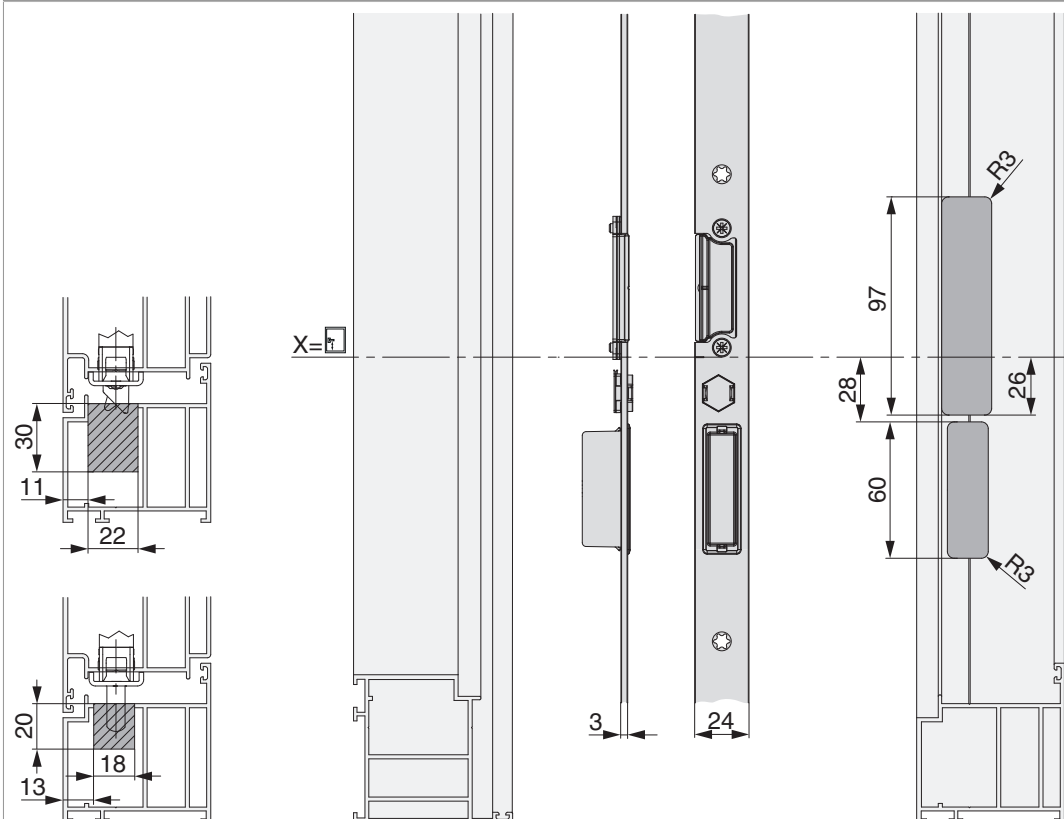
Detail C
