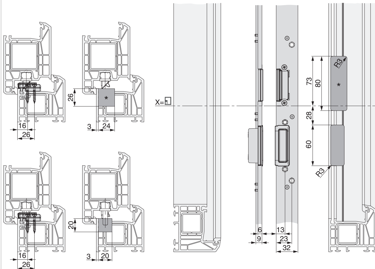
Detail B
