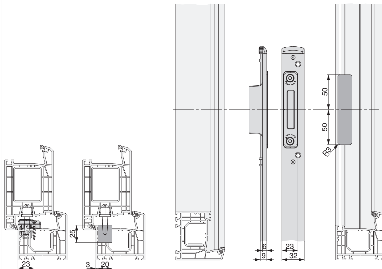
Detail A
