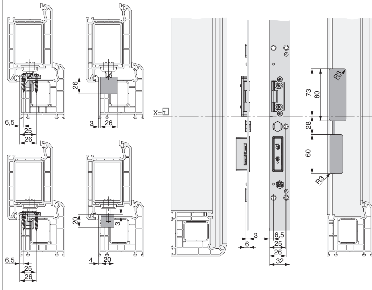
Detail B
