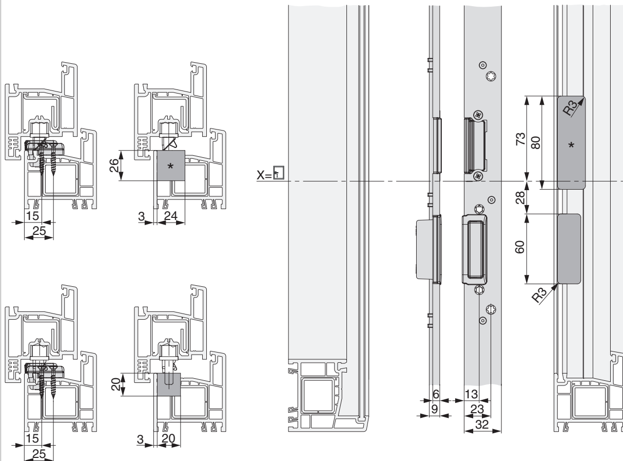
Detail B
