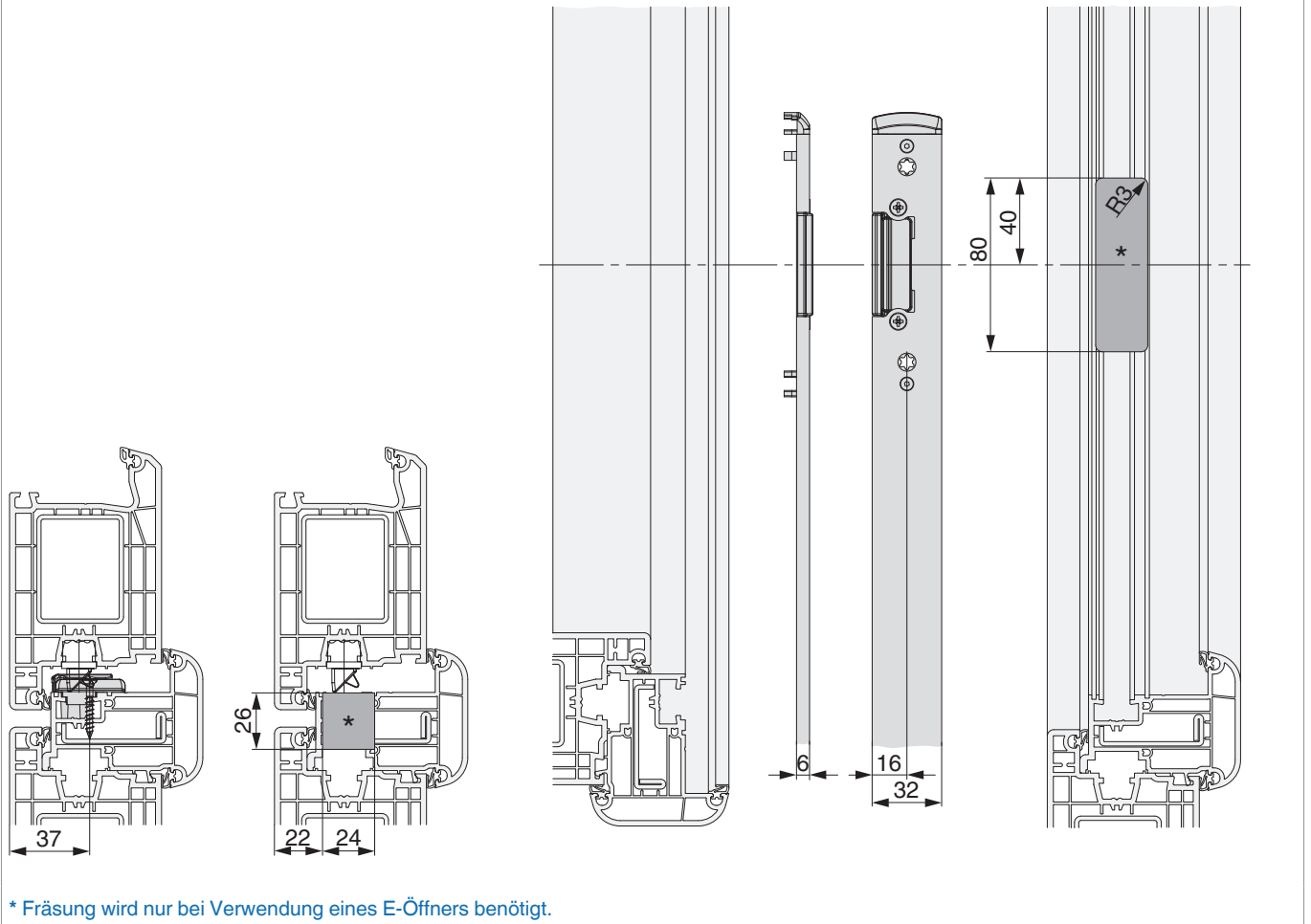
Detail C
