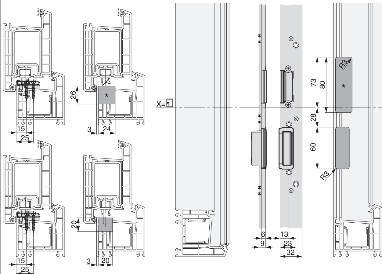
Detail B
